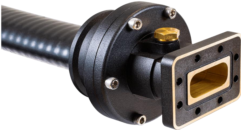
Product in use with Elliptical Waveguide
