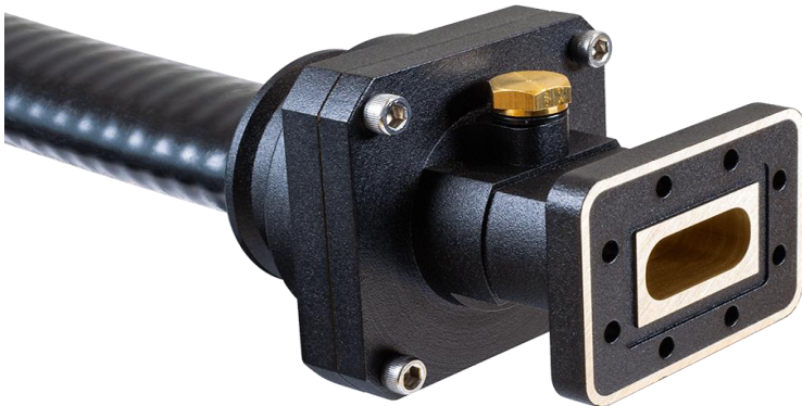
Product in use with Elliptical Waveguide
