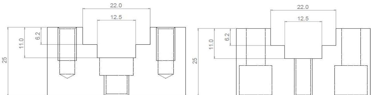
Pair of hangers in the stacked configuration
